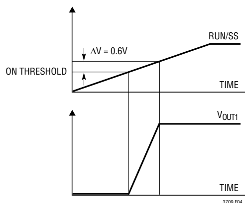
Figure 4. Monotonic Soft-Start Waveforms
