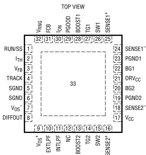
UH PACKAGE 32-LEAD (5mm x 5mm) PLASTIC QFN
