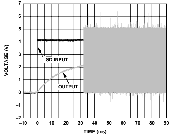
Figure 30. Turn-On Response
