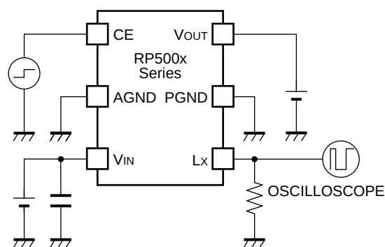
Soft-start Time
