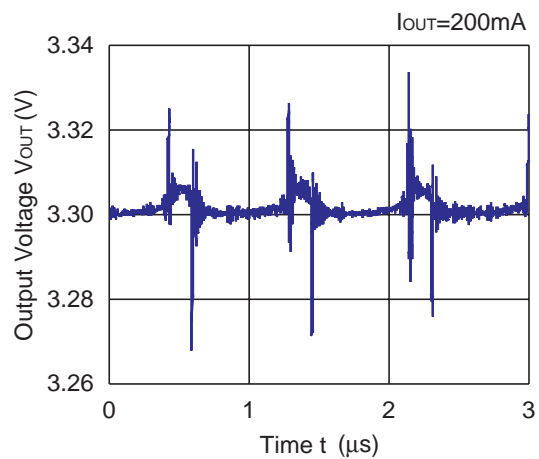
RP500x33xA
