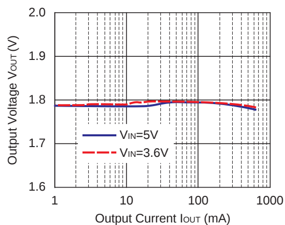
RP500x181A/183A
