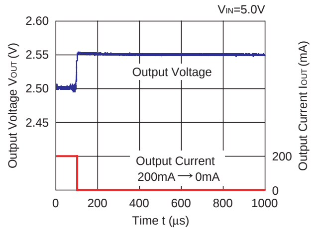
RP500x251A/253A
