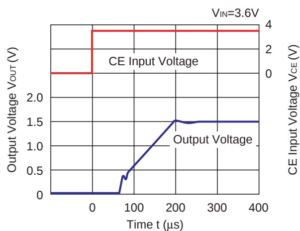
RP500x152A/154A ( I_{OUT}=1.5mA )
