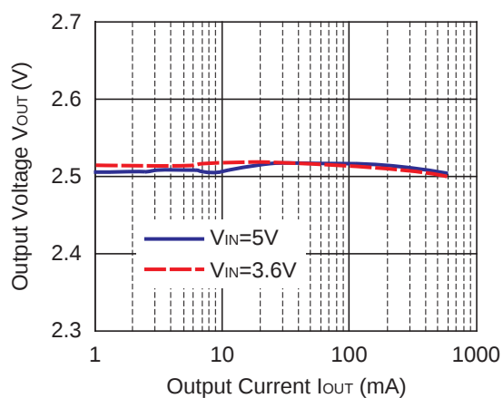
RP500x152A/154A
