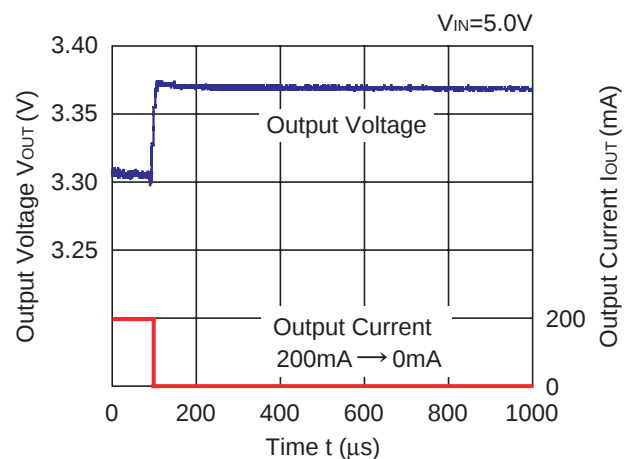
RP500x331A/333A
