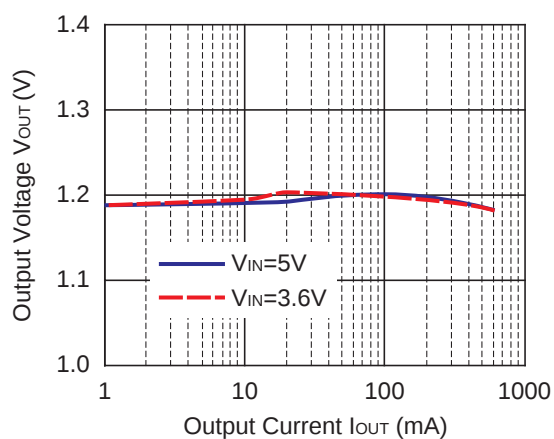
RP500x121A/123A
