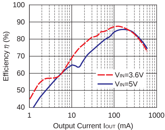
RP500x152A/154A
