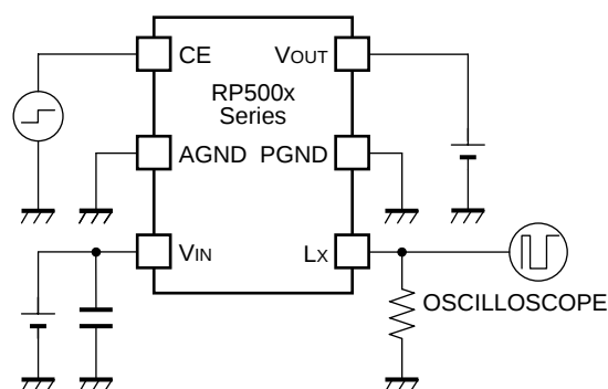
Soft-start Time
