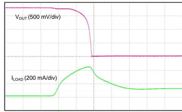
Time ( 100\text{ }\mu\text{s/div} ) TLV73318PDBV, 1\text{-}\mu\text{F} output capacitor
