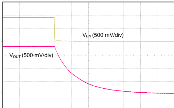
Time ( 100\text{ }\mu\text{s/div} ) TLV73318PDBV, I_{OUT} = 300\text{ mA} , 1\text{-}\mu\text{F} output capacitor
