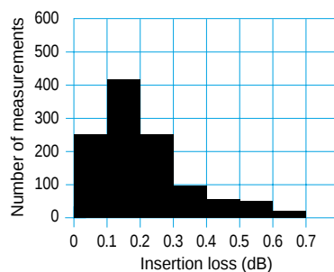
Insertion loss
