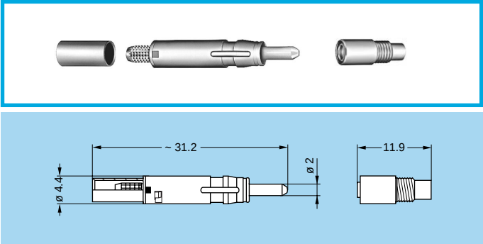
PSS.F2 Female F2 Fibre Optic Contact
