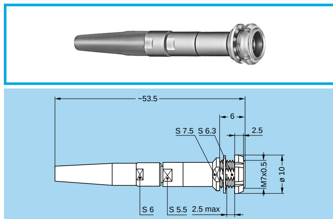
PEG.00 Fixed socket, nut fixing, key (G) or key (B), with bend relief (back panel mounting)
