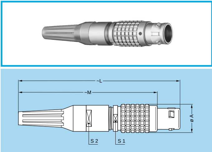
FGG Straight plug, key (G) or keys (A...L) cable collet and nut for fitting a bend relief
