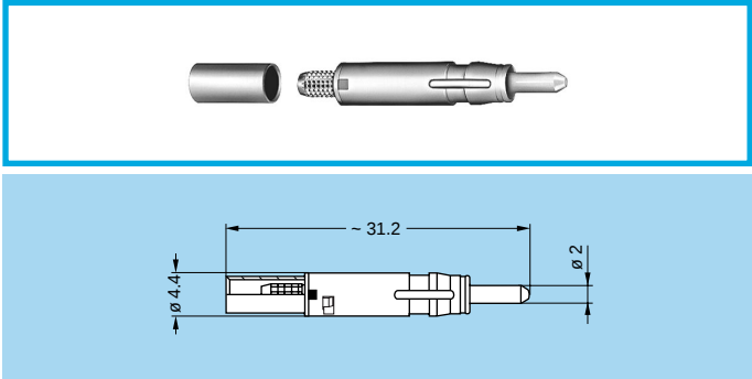
FFS.F2 Male F2 Fibre Optic Contact
