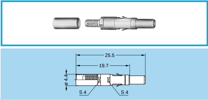
FFS Male coaxial contact type C
