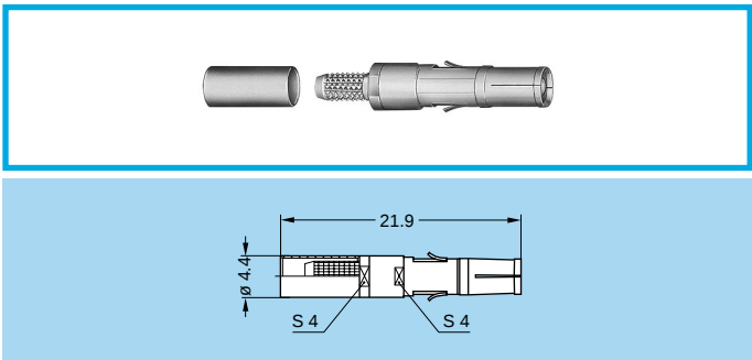
PSS Female coaxial contact type C
