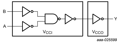
Fig. 2. Logic diagram
