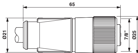
Dimensioned drawing
