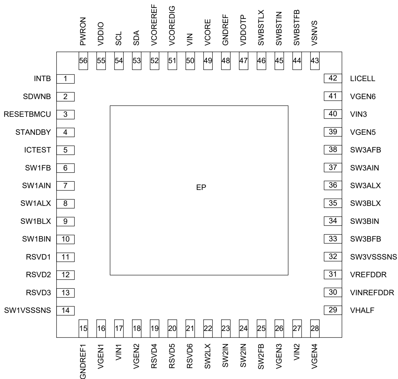
Figure 3. Pinout diagram
