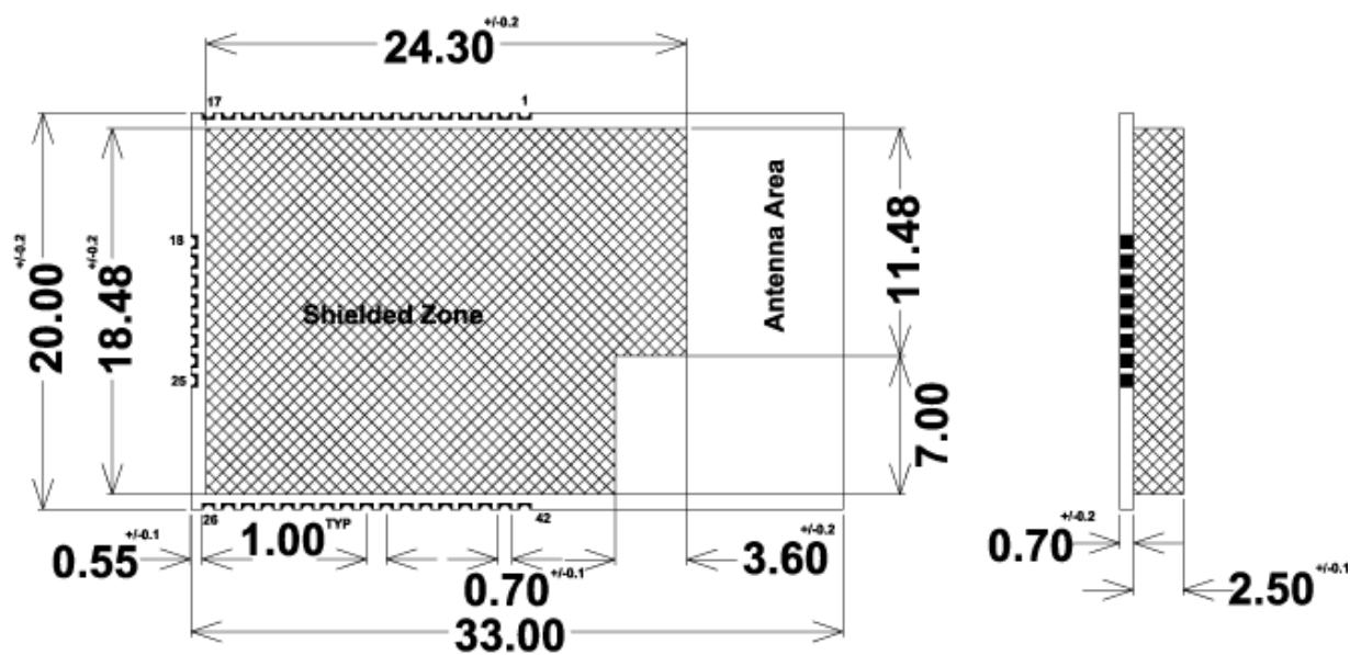
Figure 3-1. ATZB-X0-256-3-0-C Dimensions
