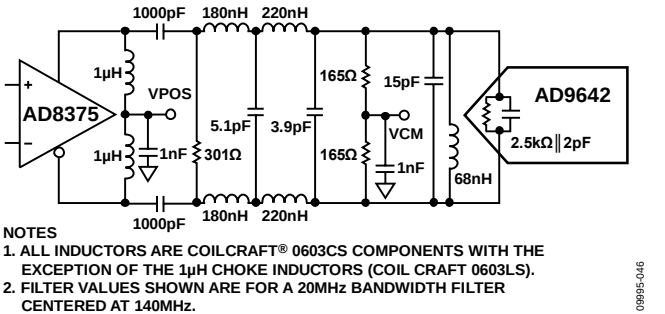
Figure 49. Differential Input Configuration Using the AD8375
