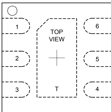
MLPD-W6; 3x3, 6 LEAD \theta_{JA} = 50^{\circ}\text{C/W}
