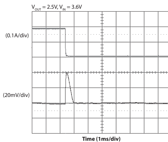
Load Transient Response (Falling Edge)
