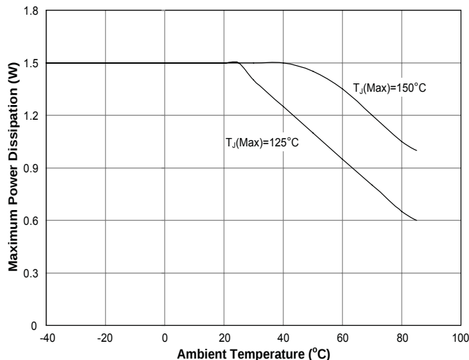
Figure 3 — Maximum P_D vs. T_A
