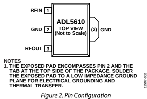
Figure 2. Pin Configuration
