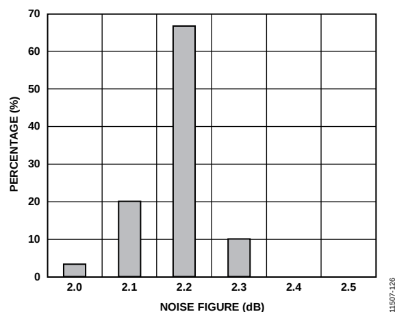
Figure 24. Noise Figure Distribution at 900 MHz
