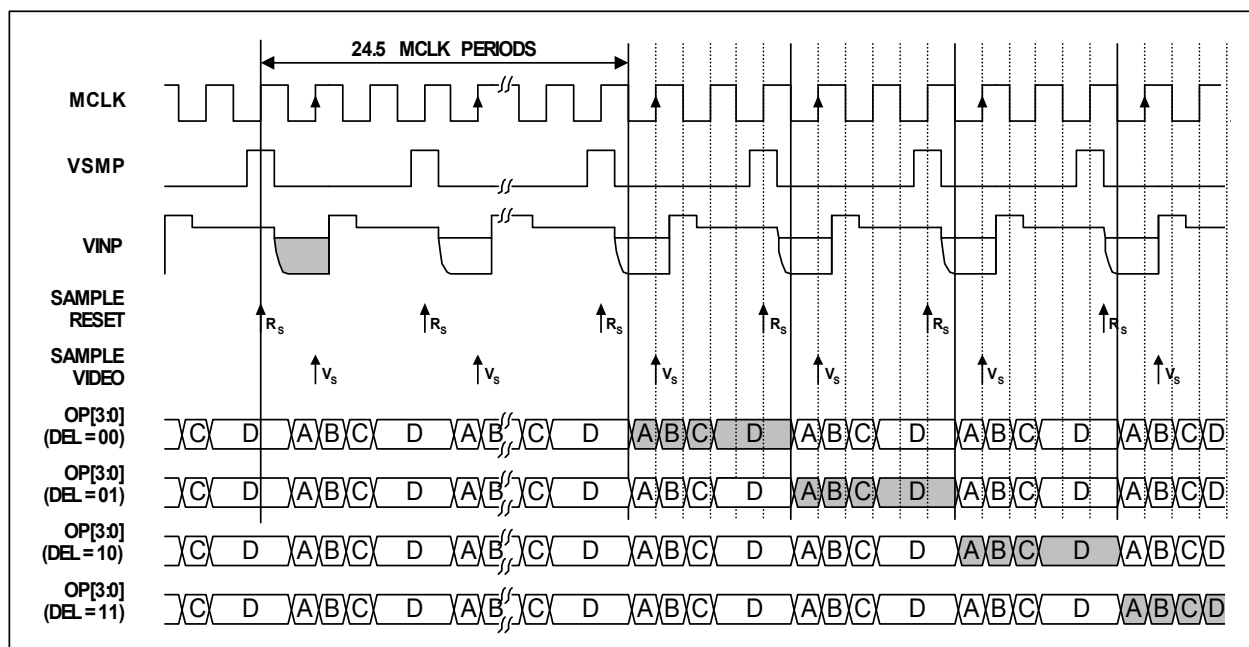
Figure 30 Mode 1 Operation
