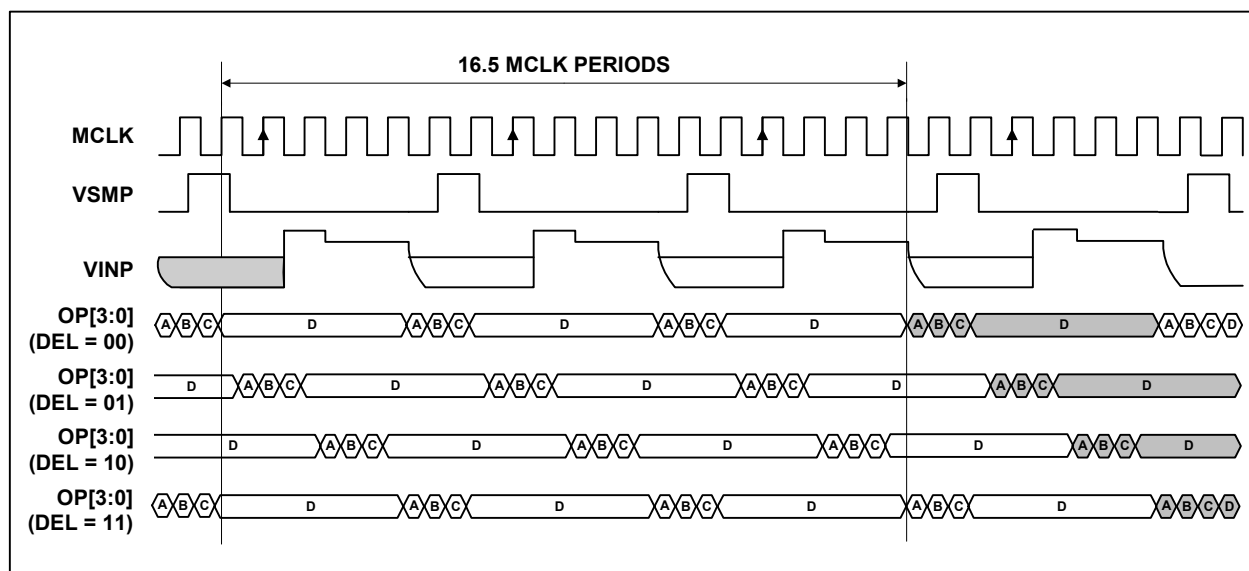
Figure 30 Mode 1 Operation
