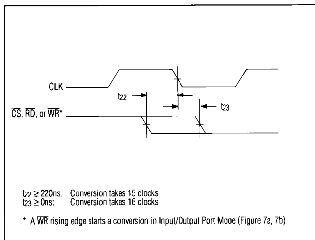
Figure 11. CS, RD, or WR to CLK Setup and Hold Time for Synchronous Operation
