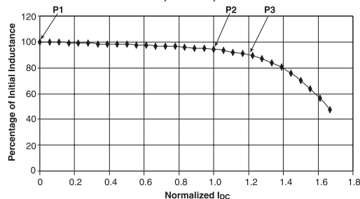
Inductance vs Current Characteristics P1681, P2005, P2004
