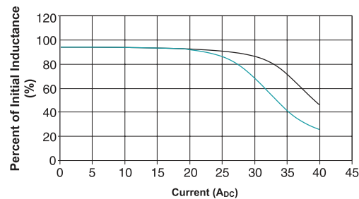
PA0229 Inductance vs. DC Current at 25°C
