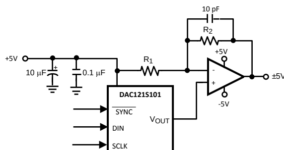
Figure 45. Bipolar Operation
