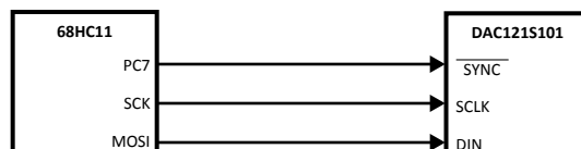
Figure 39. 68HC11 Interface
