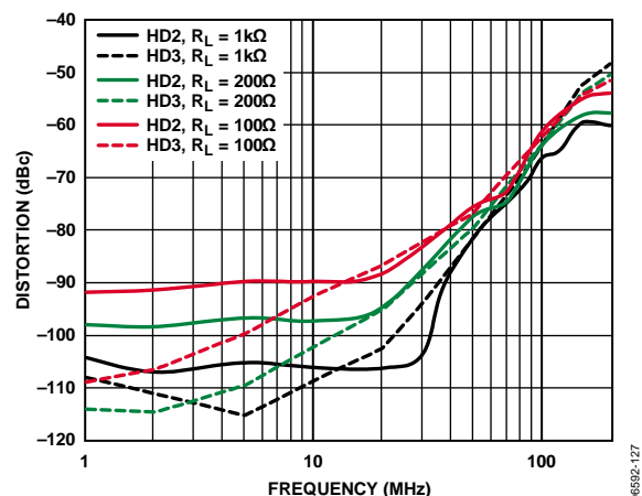
Figure 29. Harmonic Distortion vs. Frequency for Various Loads
