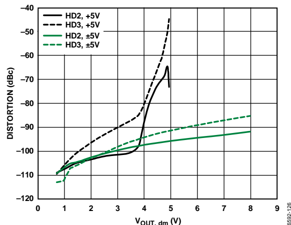
Figure 28. Harmonic Distortion vs. V_{OUT} and Supply Voltage
