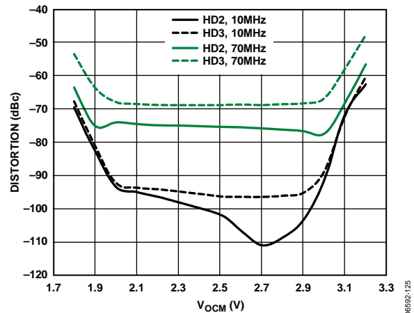
Figure 30. Harmonic Distortion vs. V_{OCM} and Frequency, V_S = 5 V
