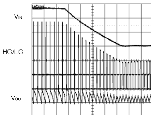
Figure 31. VIN Change (19V to 5V)
