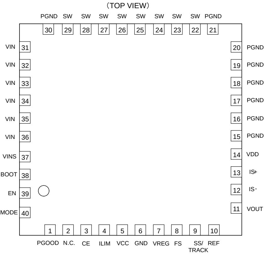
Figure 2. Pin Configuration
