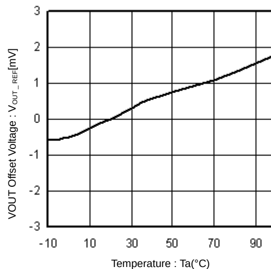
Figure 9. VOUT Offset Voltage vs Temperature
