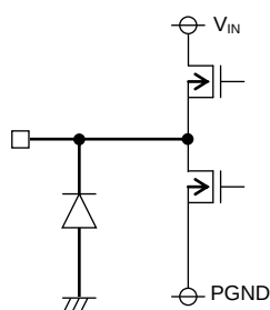
Pin 22-29 (SW)
