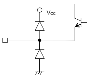
Pin 8 (FS)
