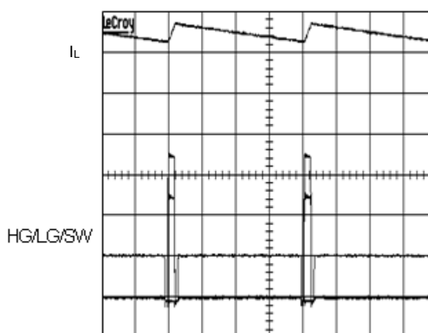
Figure 29. OCP Status ( I_O=5A )
