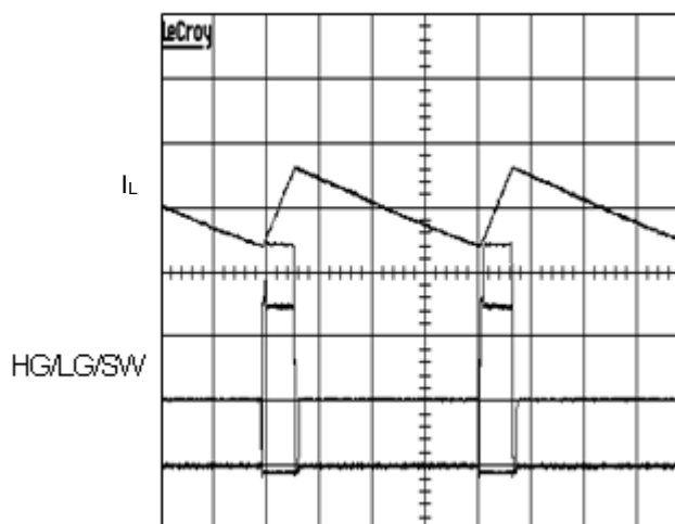
Figure 27. Continuous Mode ( I_O=0A )
