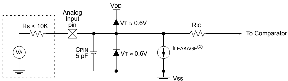
FIGURE 19-3: ANALOG INPUT MODEL
