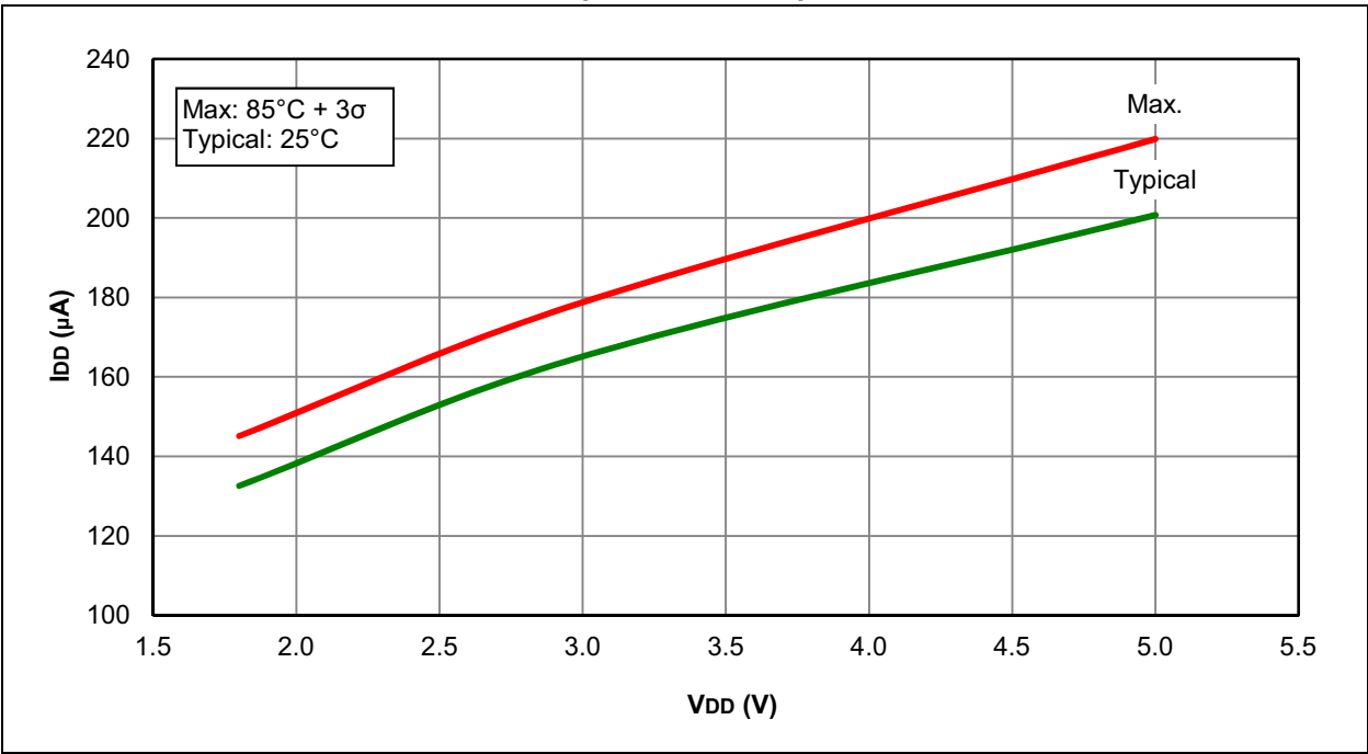
FIGURE 31-14: I_{DD} , MFINTOSC MODE ( F_{osc} = 500\text{ kHz} ), PIC16F1824/8 ONLY
