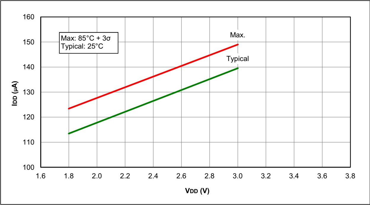
FIGURE 31-13: I_{DD} , MFINTOSC MODE ( F_{osc} = 500\text{ kHz} ), PIC16LF1824/8 ONLY
