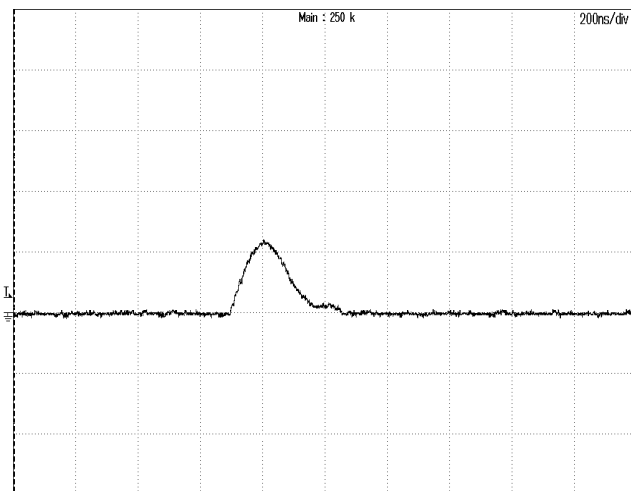
Figure 11: Inrush current @ Vin=48V CH1: i in , 2A/div, 200nS/div; Max current 2.4A, I 2t =1.24E-7 A 2 S
