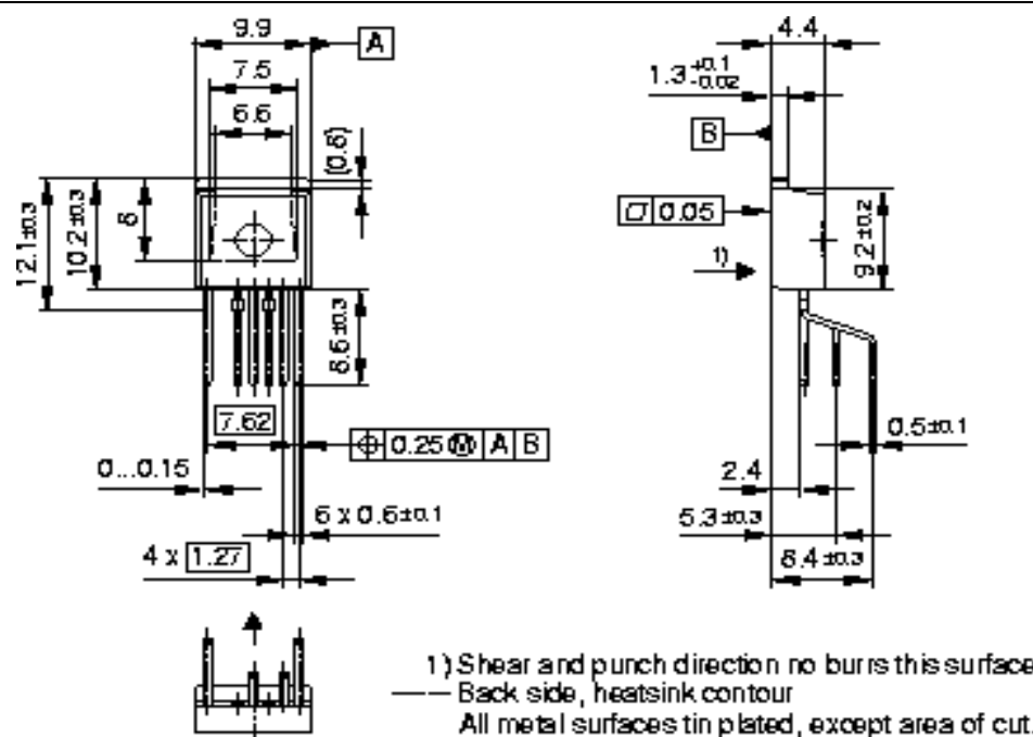
Figure 60 PG-TO220-6-46 (Isodrain Package)
