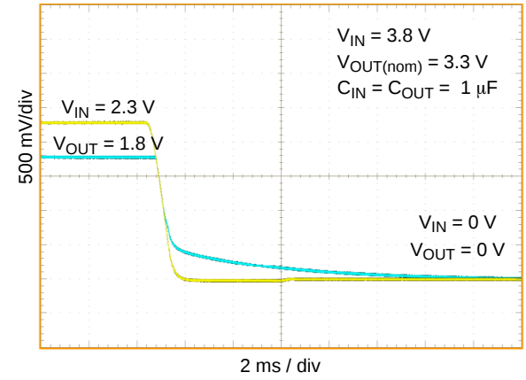
Figure 62. Enable Turn-Off Response V_{OUT} = 1.8 \text{ V} , C_{OUT} = 1 \mu\text{F} (A Version)
