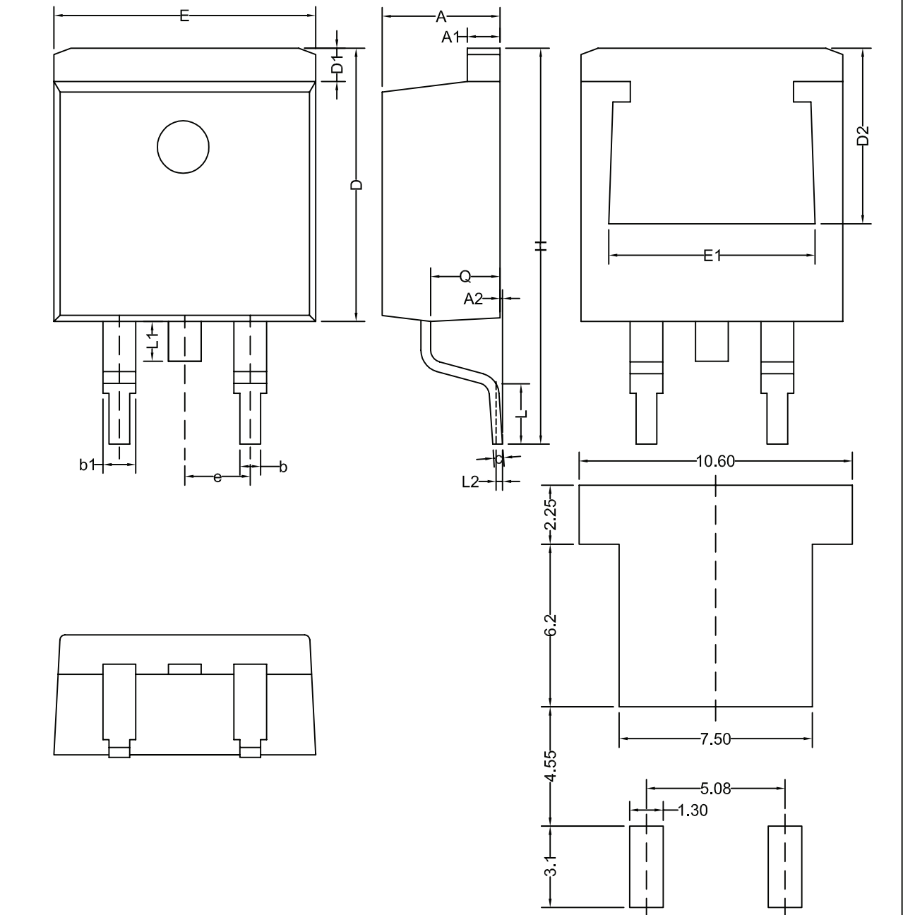
Recommended Footprint
