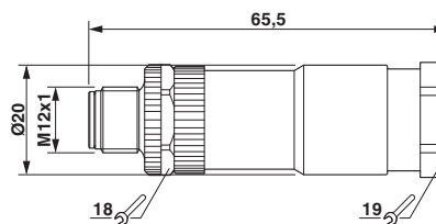
Dimensioned drawing
