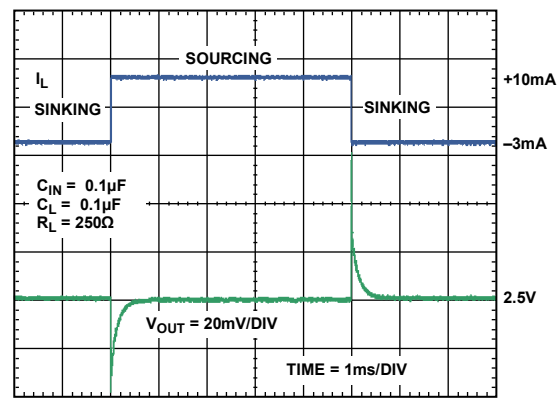
Figure 26. ADR3525 Load Transient Response
