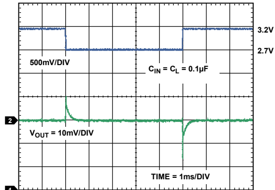
Figure 25. ADR3525 Line Transient Response
