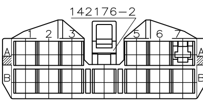
POLARIZATION TABLE (VIEW F) (tableau de detrompage)
