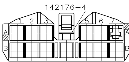
POLARIZATION TABLE (VIEW F) (tableau de detrompage)
