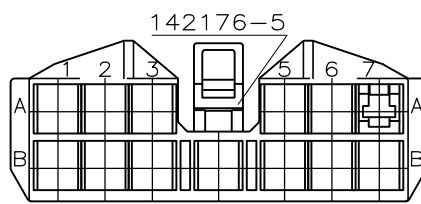
VERSION: POLARIZATIONLESS (sans detrompage) (VIEW F)
