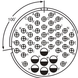
100° Rotation of 36-7
