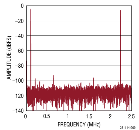
8k Point FFT, IMD, f_{SAMPL} = 5\text{Msps} , A_{IN}^+ = 100\text{kHz} , A_{IN}^- = 2.2\text{MHz}
