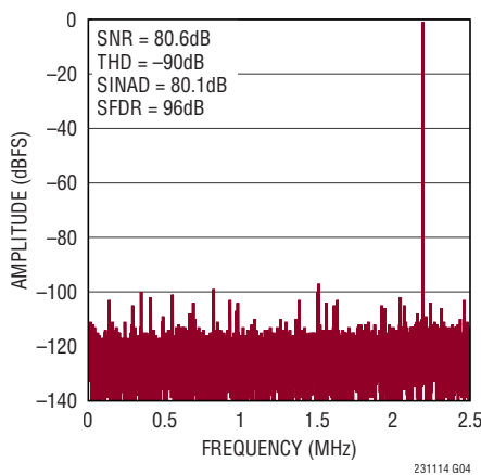
32k Point FFT, f_{SAMPL} = 5\text{Msps} , f_{IN} = 2.2\text{MHz}
