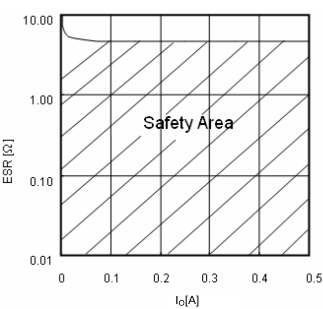
Fig.19 ESR condencer
