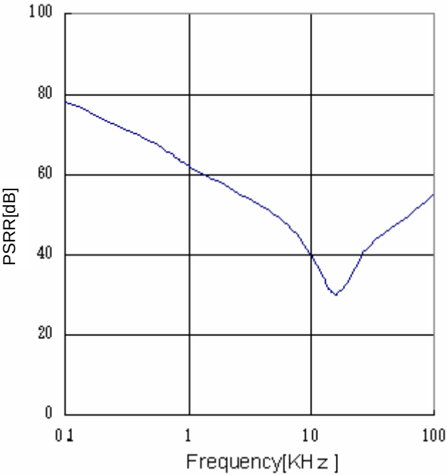
Fig.21 PSRR ( I_o=0mA )
