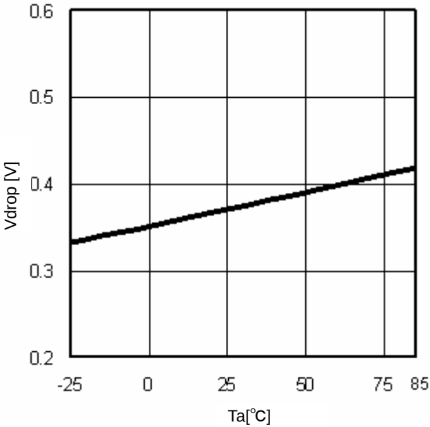
Fig.18 Minimum dropout Voltage1 ( V_{CC}=5V , I_O=-0.5A )
