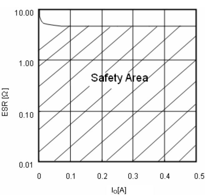
Fig.19 ESR condencer
