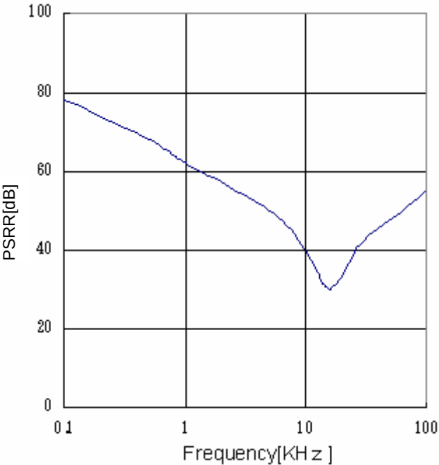
Fig.21 PSRR ( I_o=0mA )
