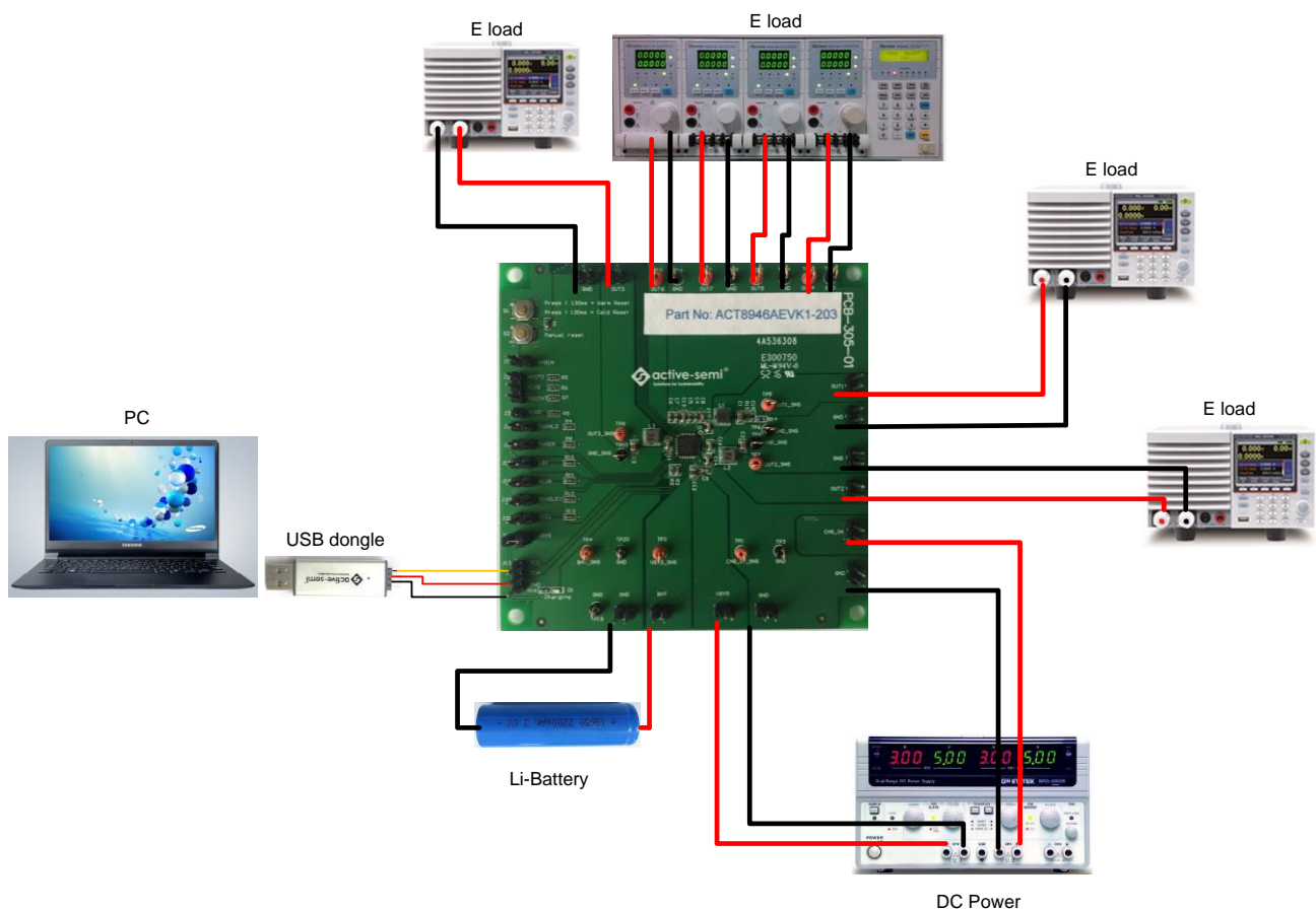
Figure 2 – EVK Setup
