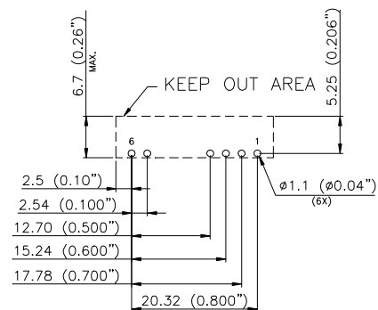
RECOMMENDED PWB PAD LAYOUT
