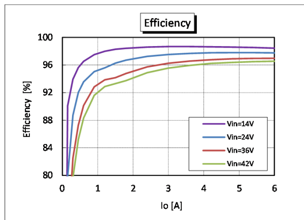
Vo vs. Line Voltage and Load Current @ +25degC. (Vo = 12V)
