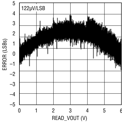
ADC READ_VOUT-INL
