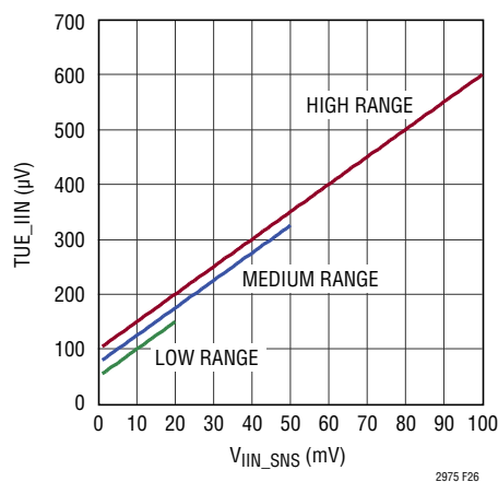
Figure 26. TUE_IIN vs READ_IIN Input Voltage in μV
