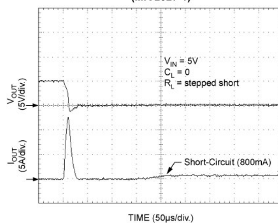
Current-Limit Response (MIC2027-1)
