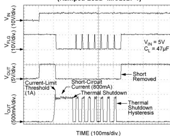
Current-Limit Response (Ramped Load—MIC2027-1)
