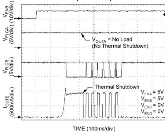
Independent Thermal Shutdown (MIC2027-1)
