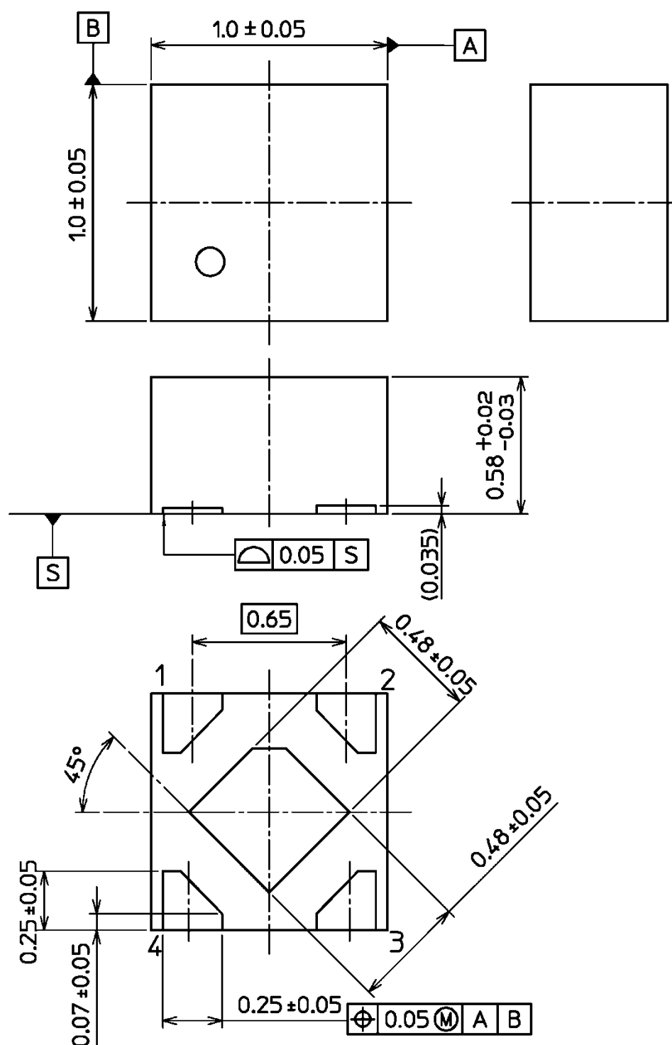
BOTTOM VIEW
