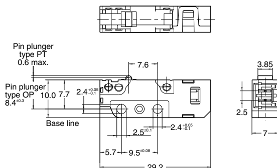
External dimensions
