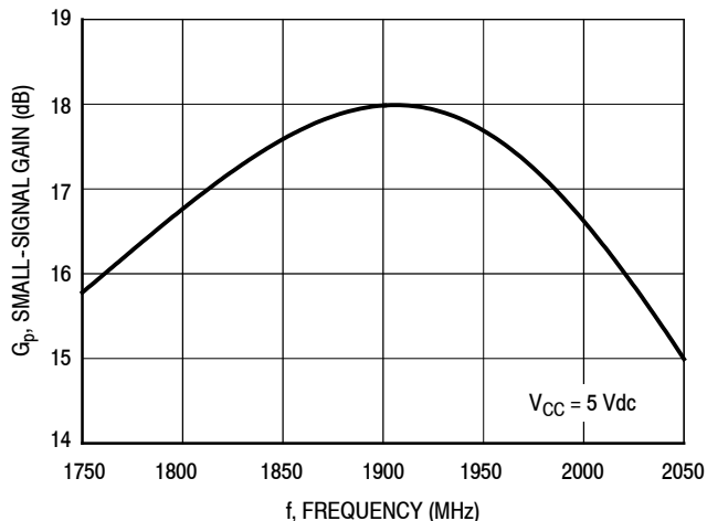
Figure 22. Small-Signal Gain (S21) versus Frequency
