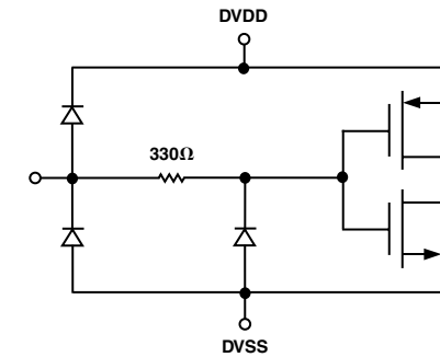
Figure 3. Digital Inputs
