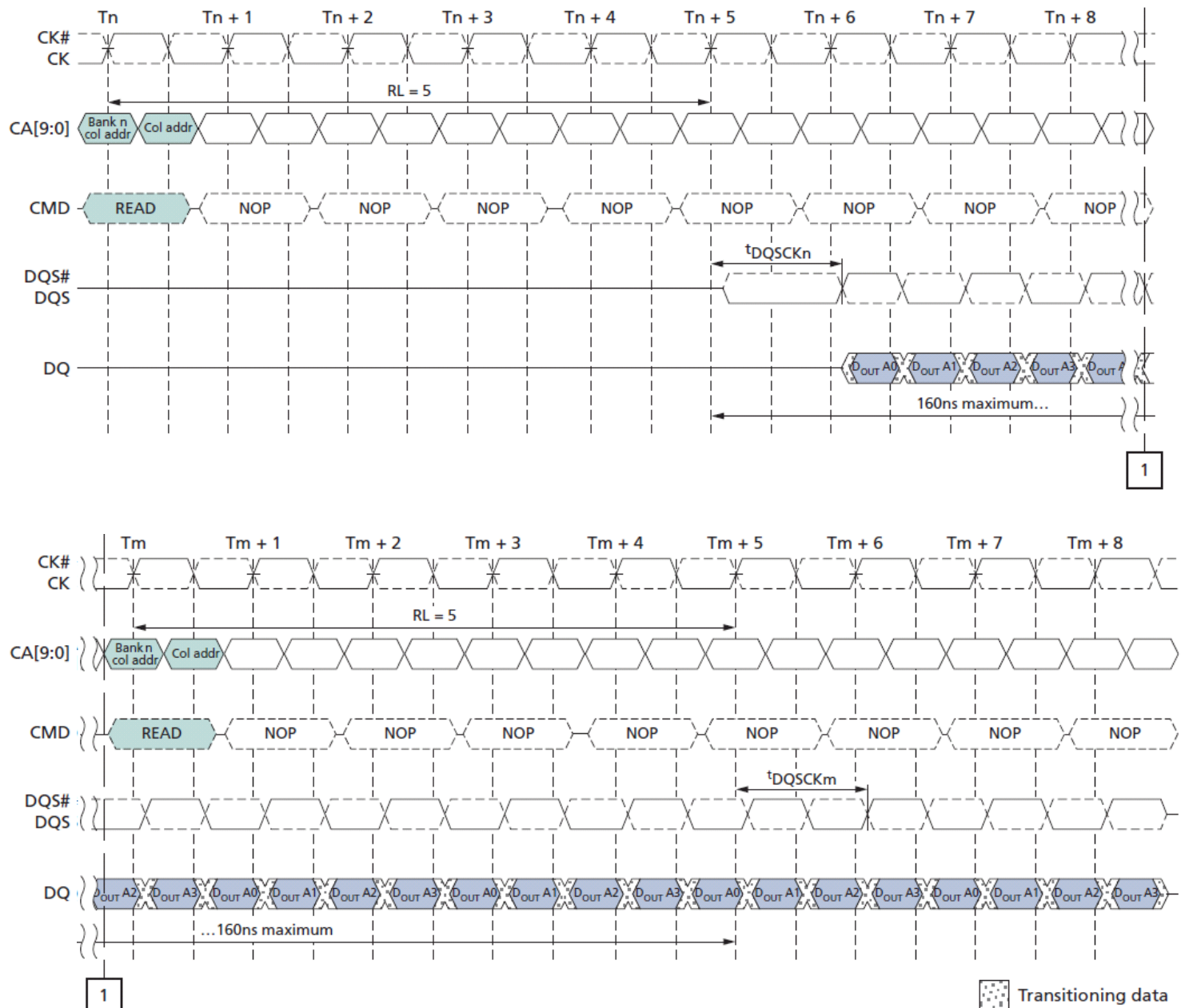
Figure 10 : tDQSKDS Timing
