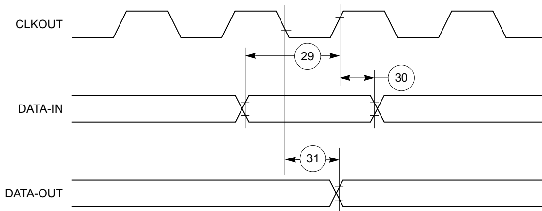
Figure 38. Parallel I/O Data-In/Data-Out Timing Diagram
