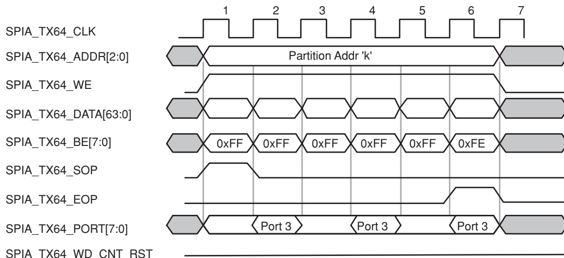
Figure 13. Basic 64-Bit Data Write Protocol to DPRAM
