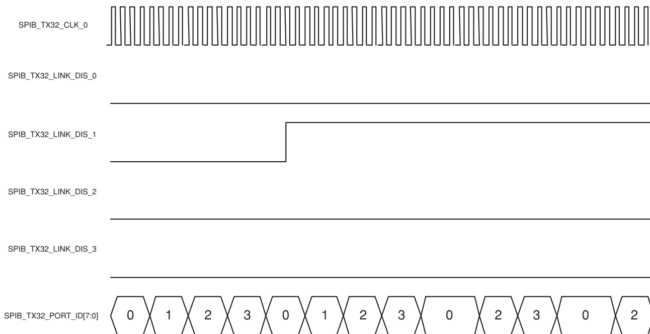
Figure 16. Port 1 Disable
