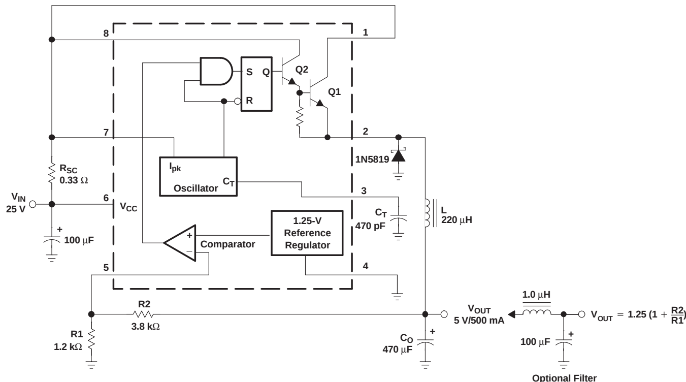
Figure 8. Step-Down Converter
