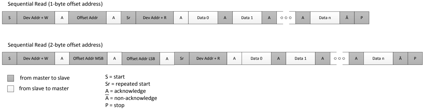
Figure 6. I 2 C Master Read Cycle Sequencing
